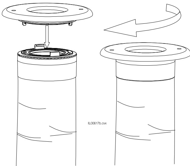
Figure 2. Installing Outlet (A) to Duct (B)
