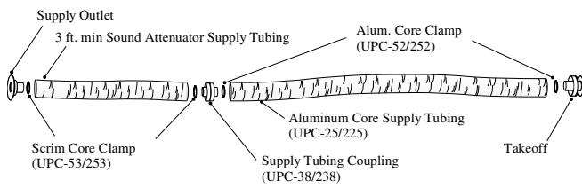
Method B (for 6 to 50 ft. runs)
