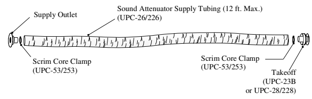
Method A (for 6 to 12 ft. runs)
