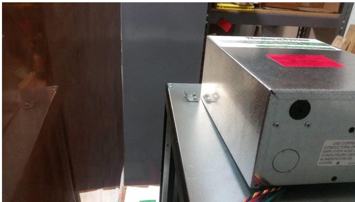
Figure 10-6 Electrostatic Discharge Test Setup VCP
